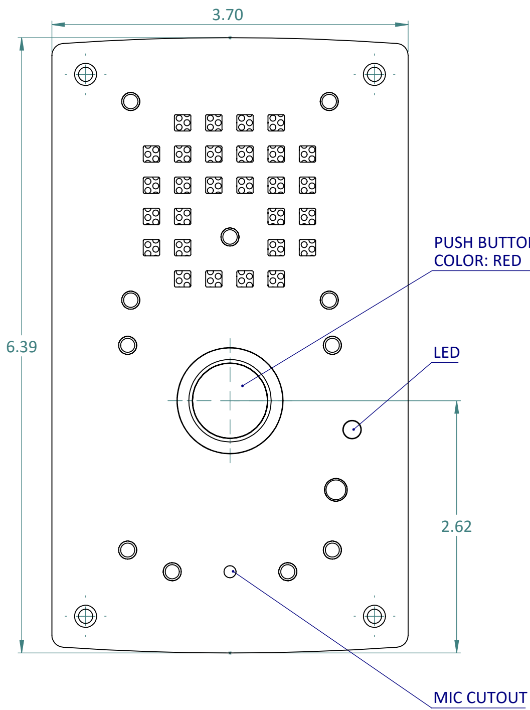
FRONT VIEW
