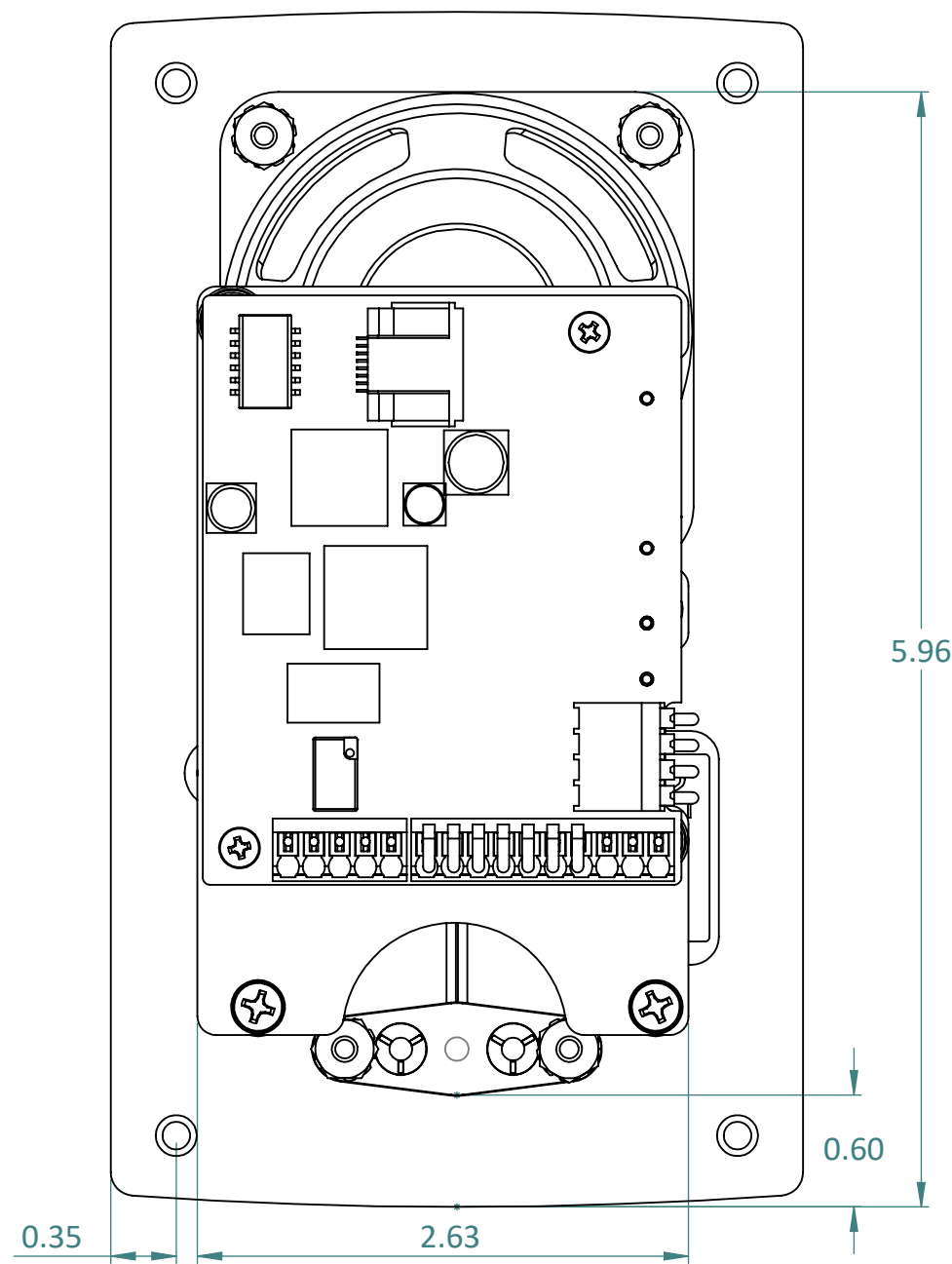
BACK VIEW
