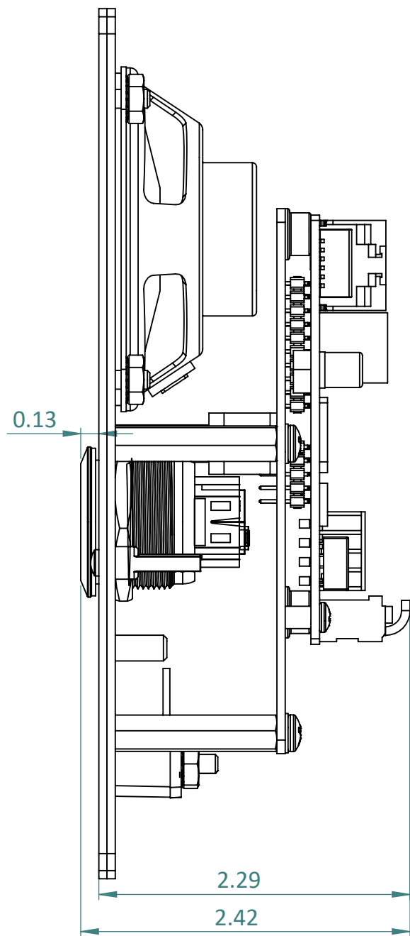
SIDE VIEW
