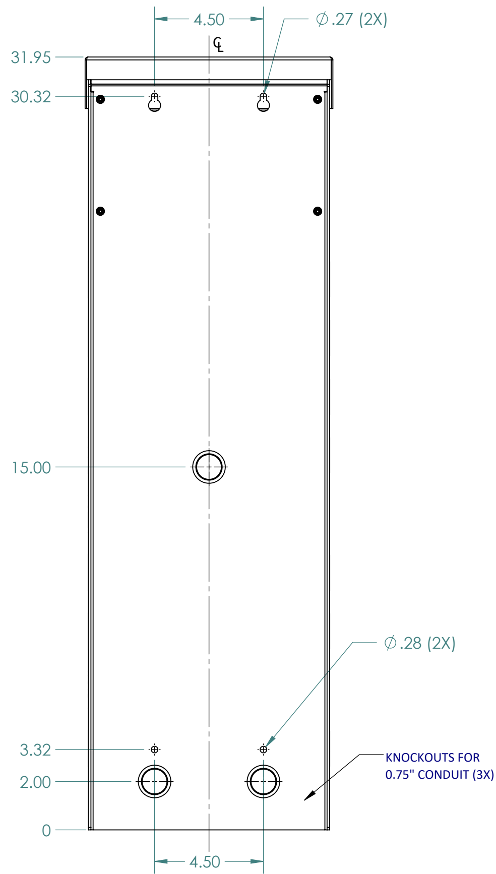
REAR VIEW
