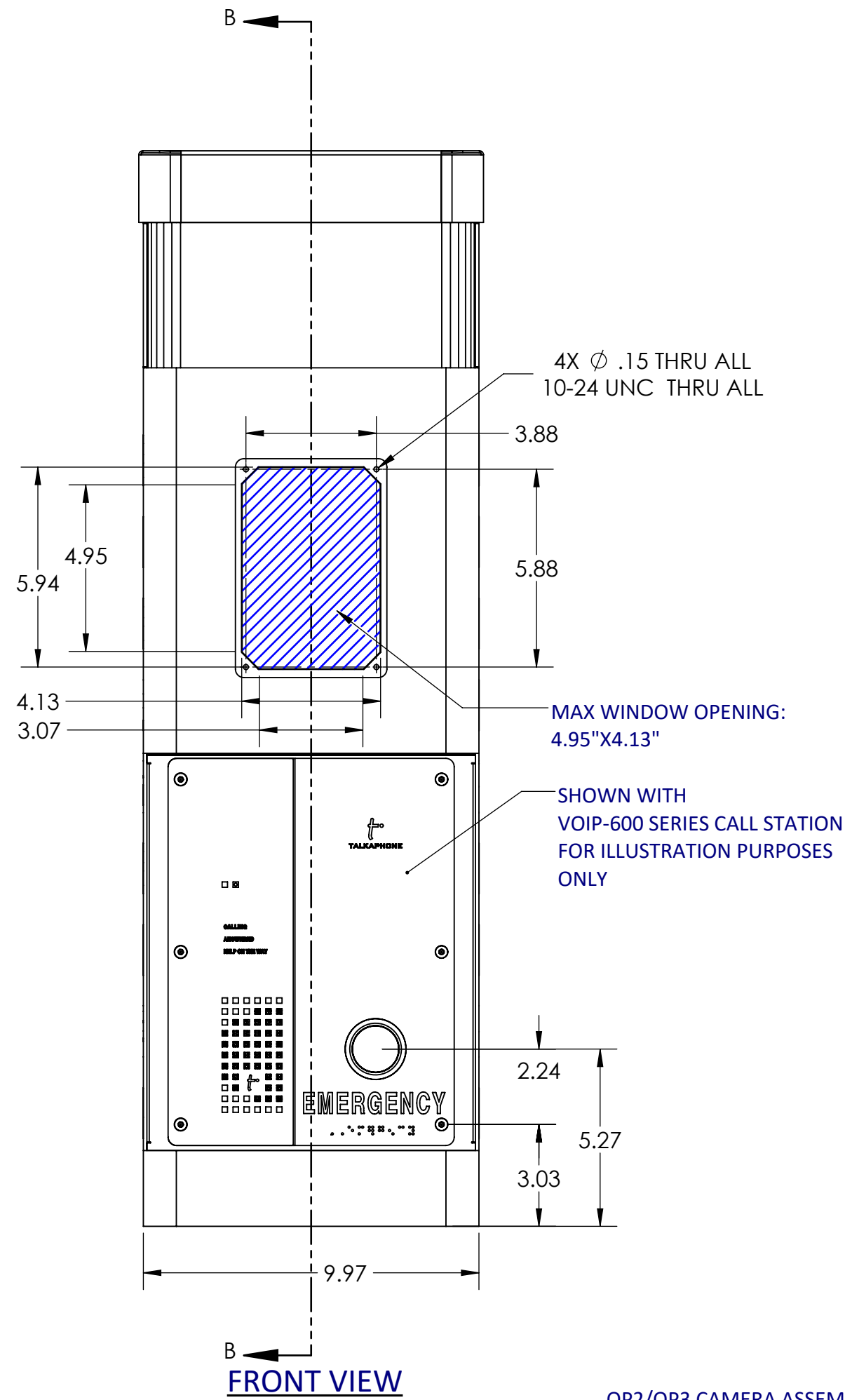
OP2/OP3 CAMERA ASSEMBLY
