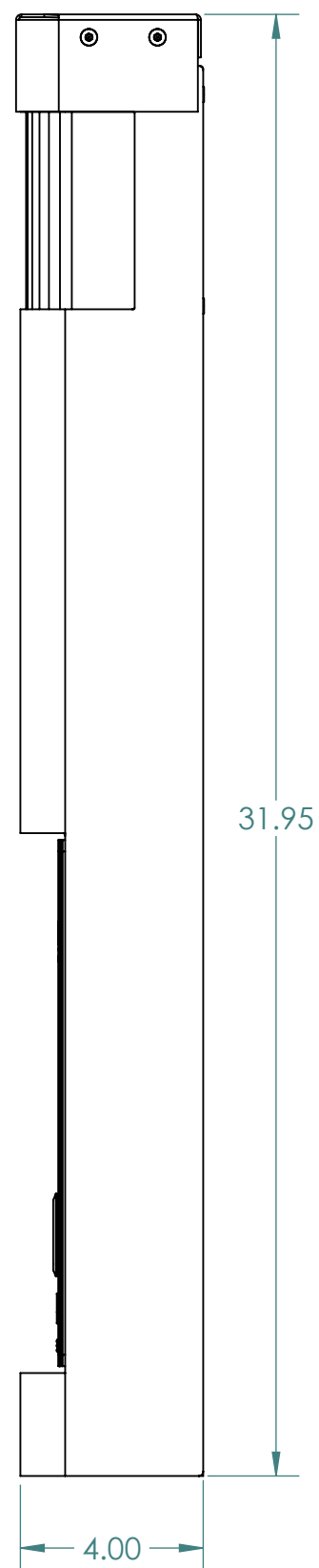
SIDE VIEW
