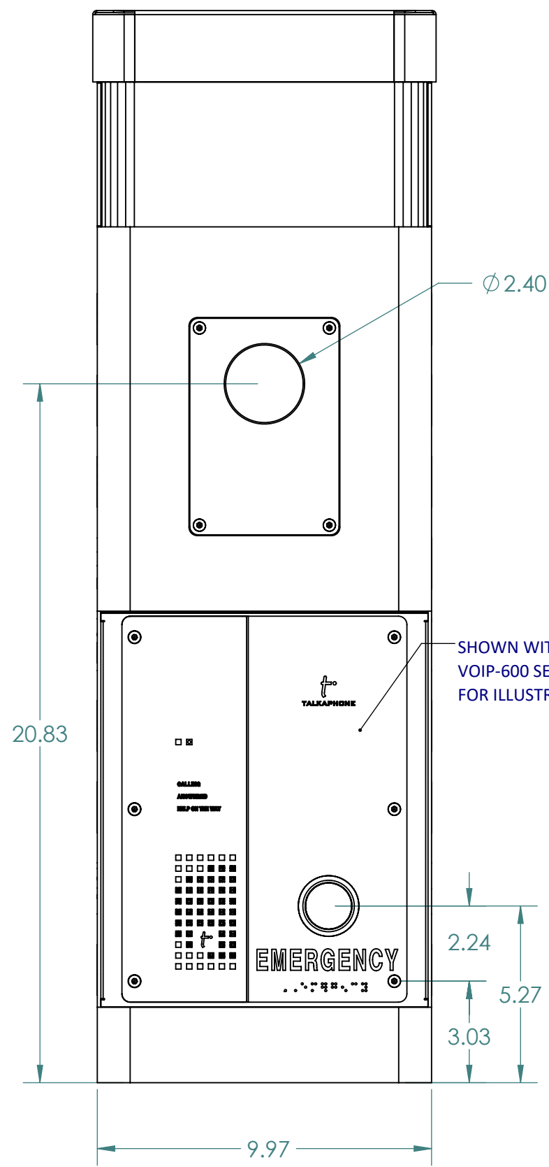
FRONT VIEW
