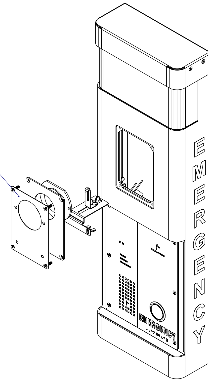
OP2/OP3 CAMERA ASSEMBLY
