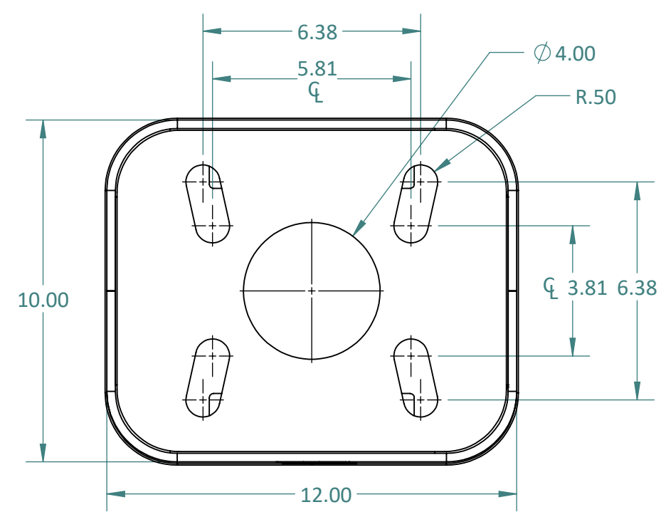
FOOT PRINT
