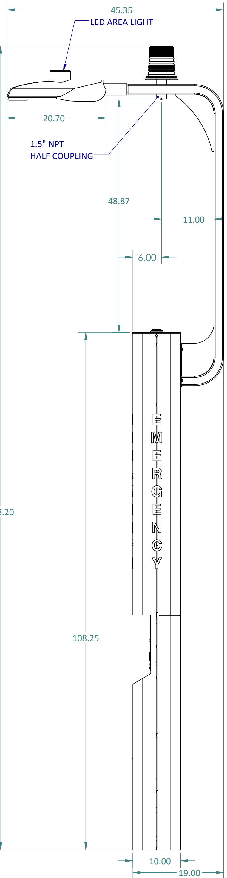
SIDE VIEW
