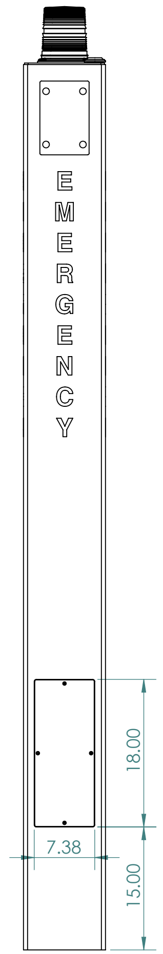
REAR VIEW
