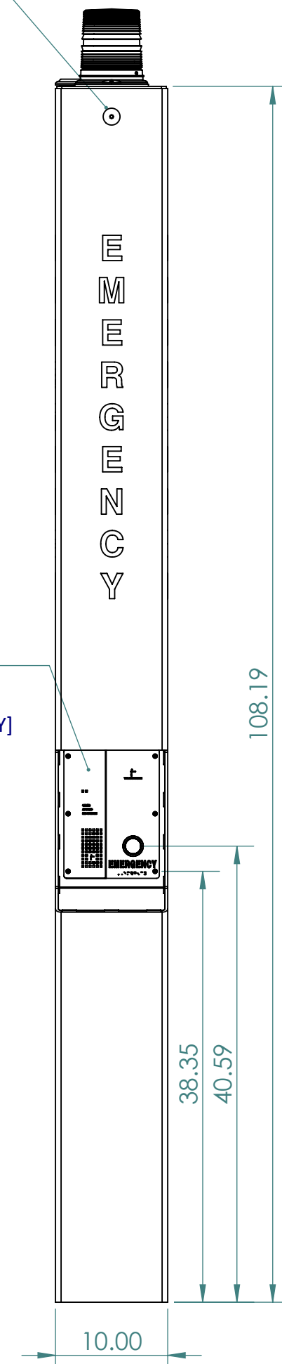
FRONT VIEW
