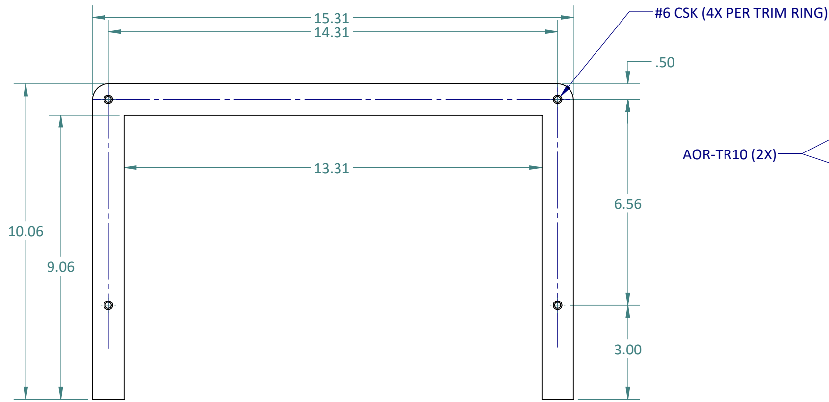
FRONT VIEW
